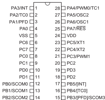
HT48R0662 28 SKDIP-A/SOP-A/SSOP-A
