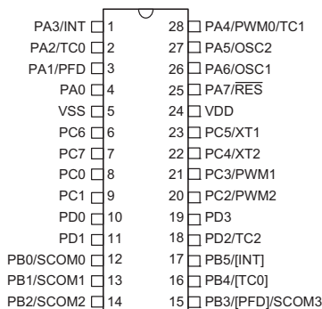
HT48R067 28 SKDIP-A/SOP-A/SSOP-A
