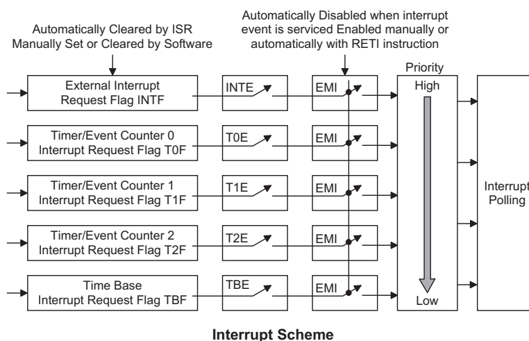
Interrupt Scheme
