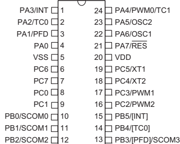
HT48R067 24 SKDIP-A/SOP-A/SSOP-A
